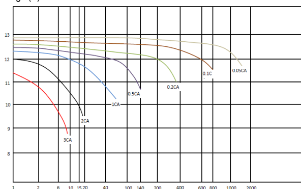
Discharge Curves at Different Discharge Rate (25°C) Voltage (V)
