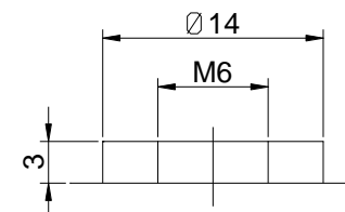
Terminal T9
